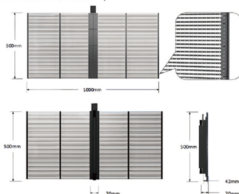
SKETCH:1000*500mm
